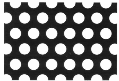
R5,00 T8,00 35%
