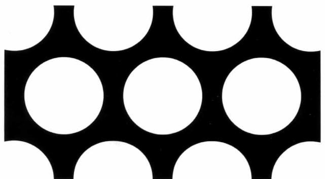
R20,0 T25,0 58%
