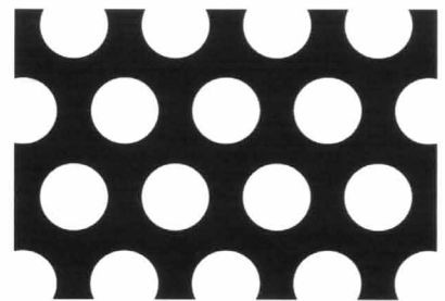
R8,00 T12,0 40%
