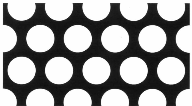
R12,0 T16,0 51%
