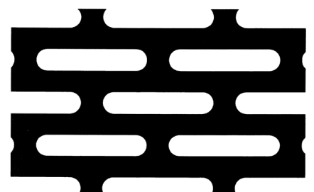
LR4,0x20,0 Z16,0/24,0 23%
