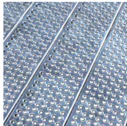
OPTIMO 05 steel heel proof pattern: dia. 5/5 mm
